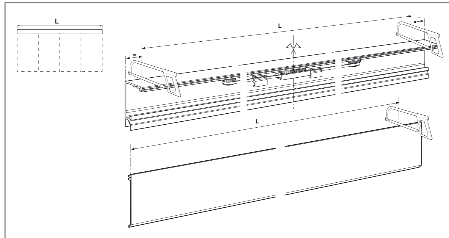
A ROLMATIC COMPAK® V12
