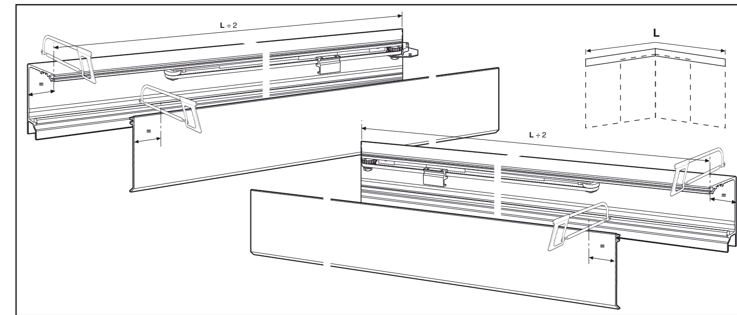
A ROLMATIC CORNER® V12
